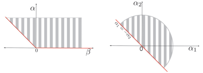
Figure 1: Parameter Space for \beta (left) and \alpha (right).
