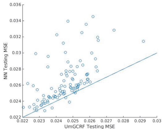
Figure 5: Scatter Plot of MSE for NN and UmGCRF, line represents equal
